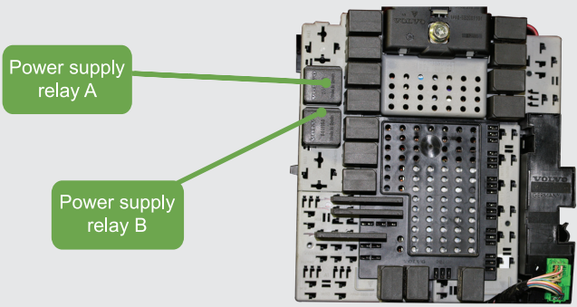
Fig. 2 Central Electronic Module
